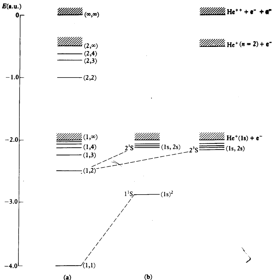
6.5 (a) The energy spectrum given by expression [6.32] with Z = 2 . The levels are labelled by (n_1, n_2) .
